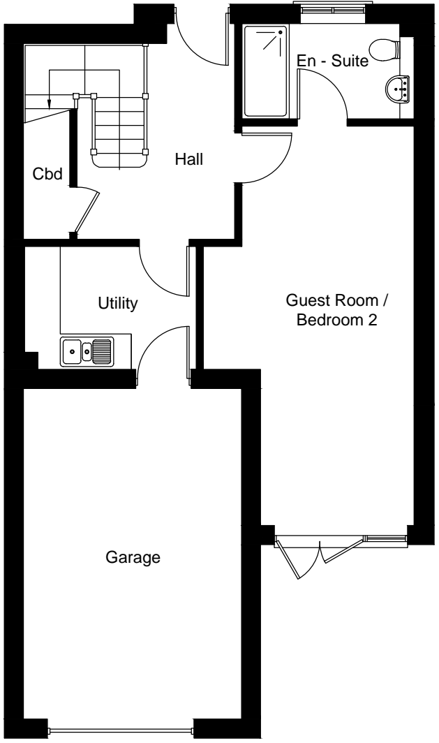
Ground Floor Plot 22
