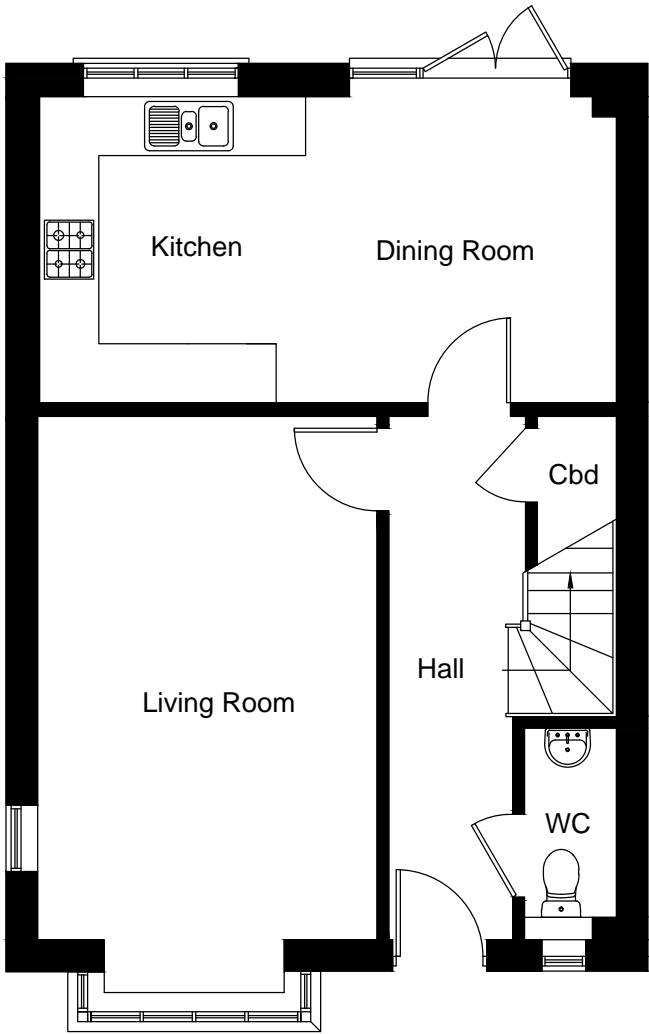
Ground Floor Plot 24
