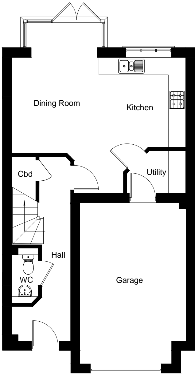
Ground Floor Plot 28
