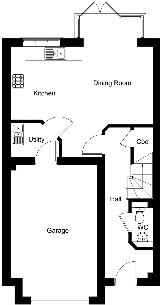
Ground Floor Plot 3
