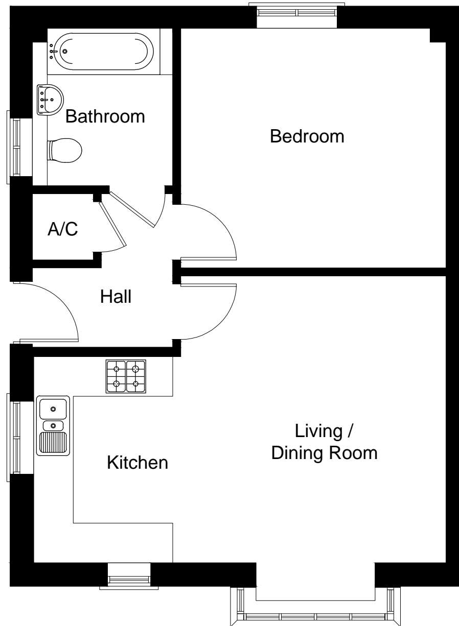
Ground Floor PLOT 32
