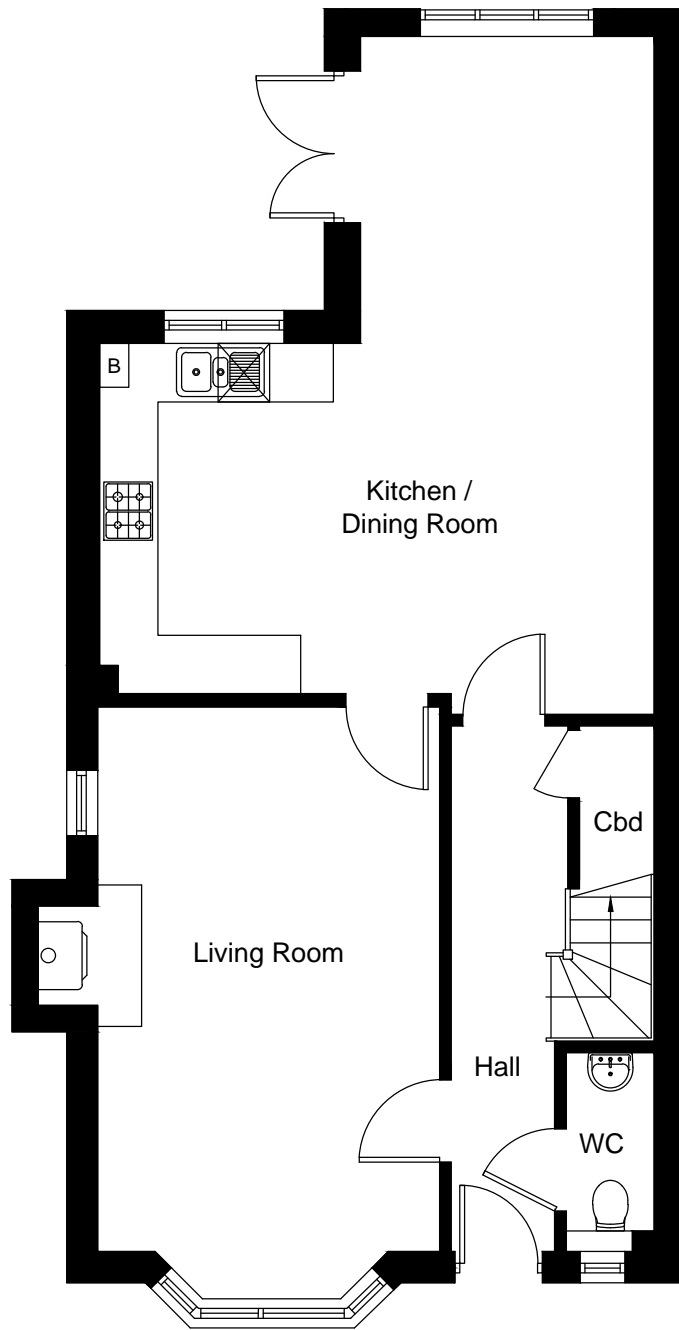
Ground Floor Plot 14
