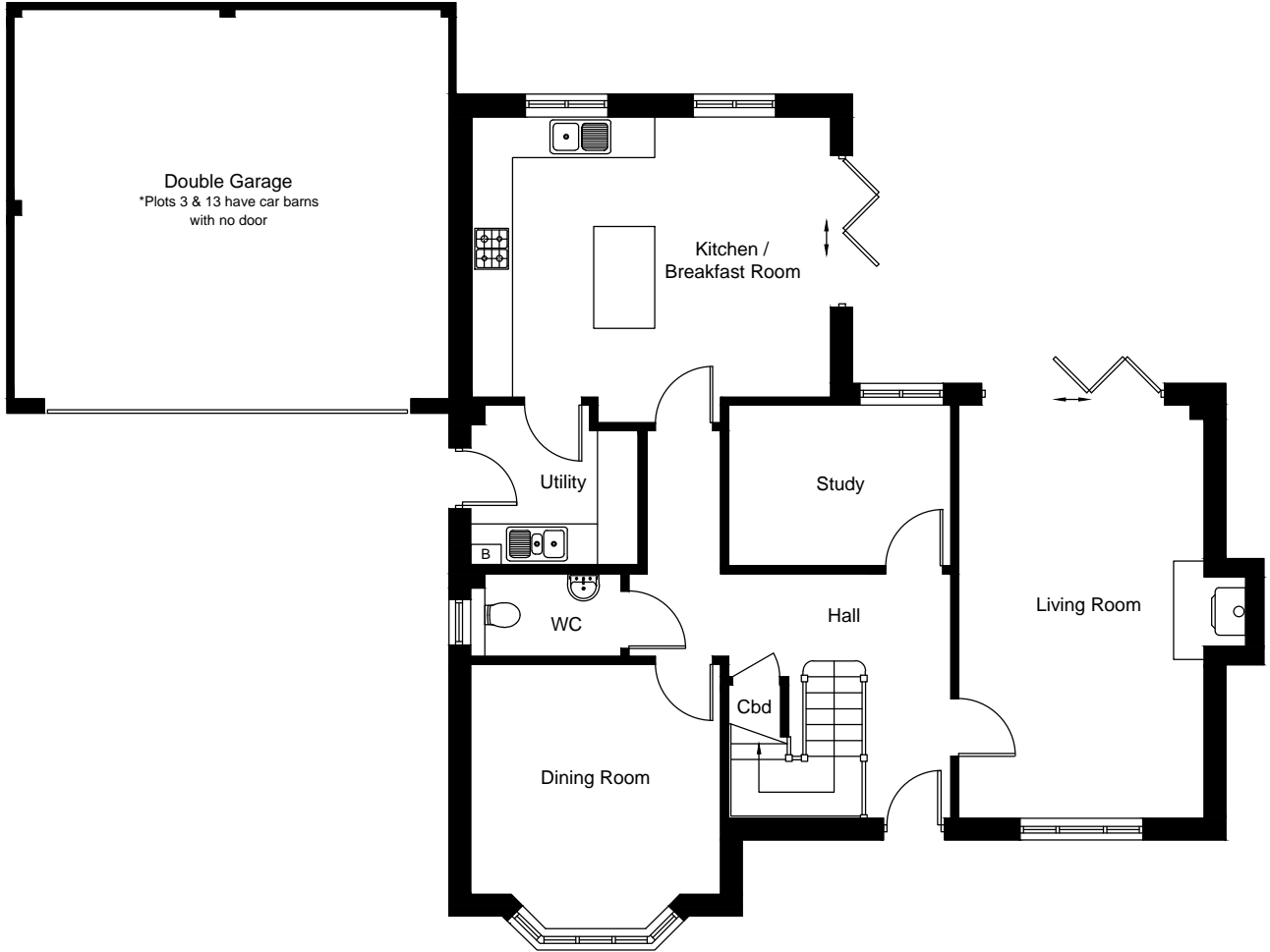
Ground Floor Plot 4
