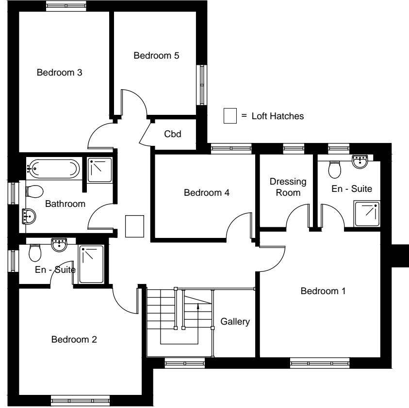
First Floor
