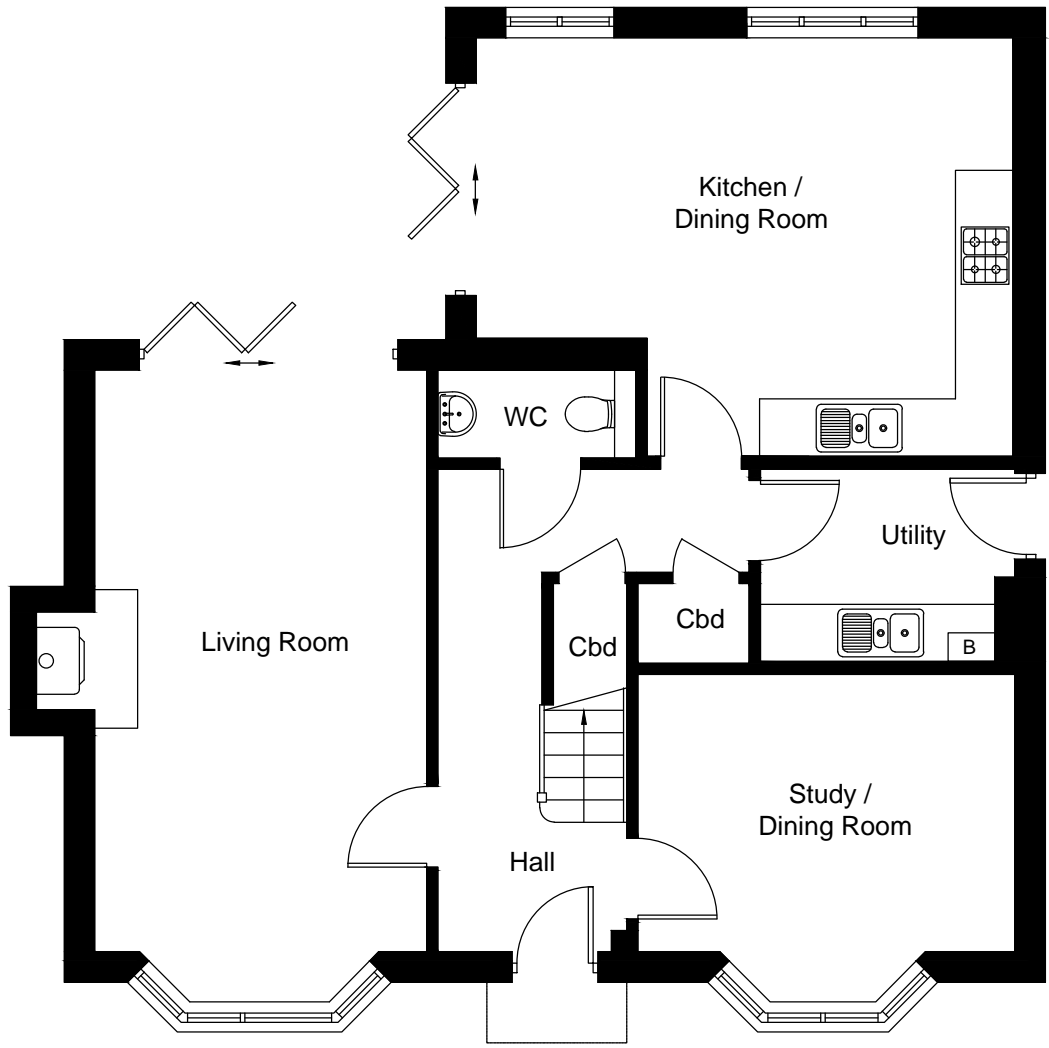
Ground Floor Plot 6
